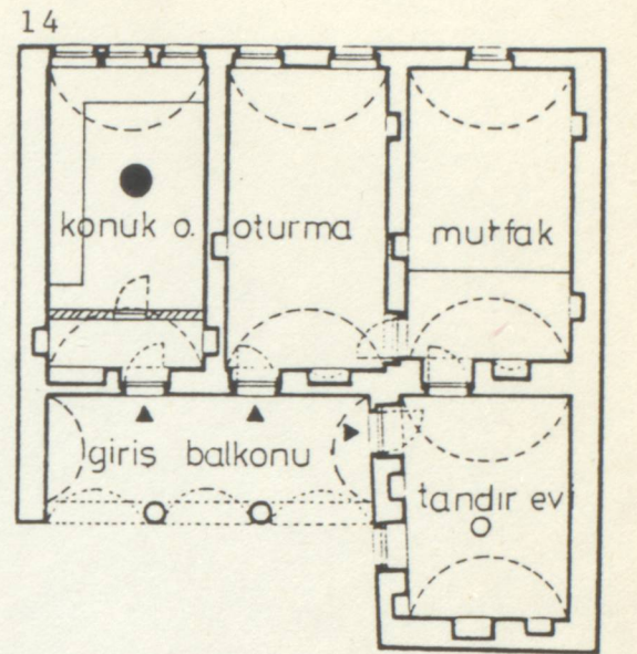
0 5M GİRİŞ KATI PLANI
