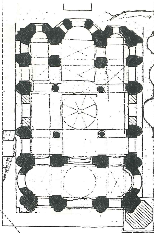
Plan
