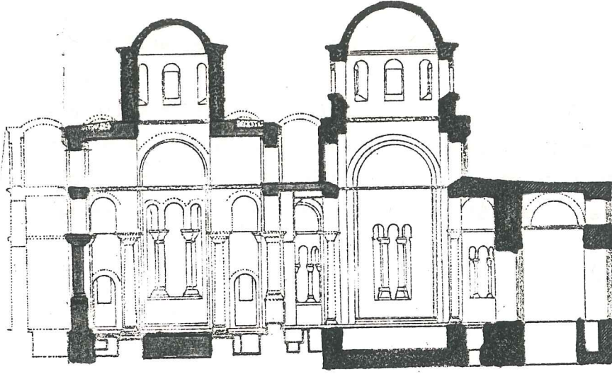
Enine kesit
