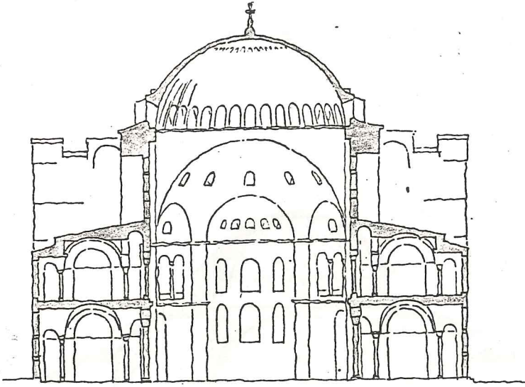
Enine kesit
